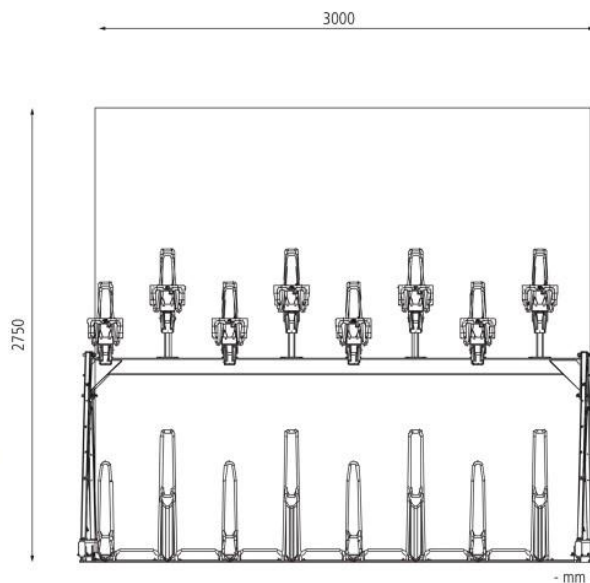
Doppelstockparker
